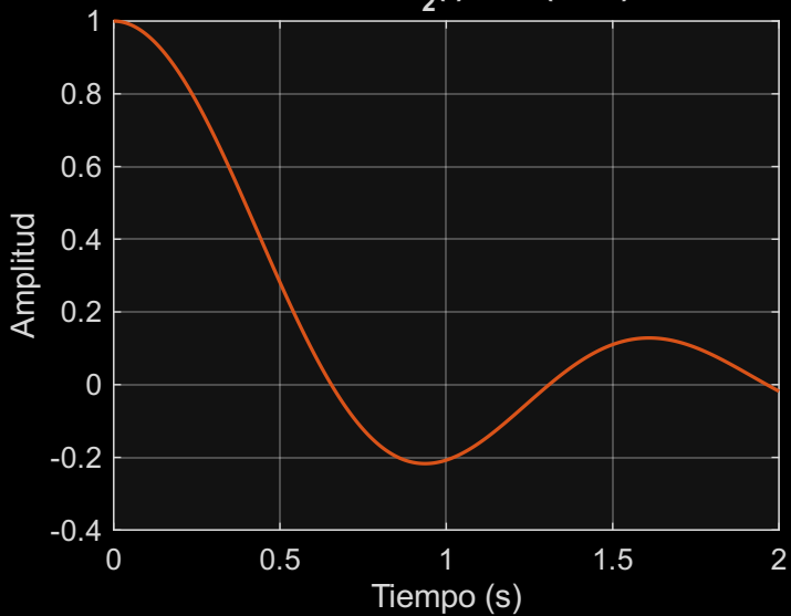
Senal continua: x_2(t) = \text{Sa}(2 \times t) , X=2.4
