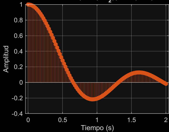
Senal discretizada (stem): x_2(t) = \text{Sa}(2 \times t) , X=2.4
